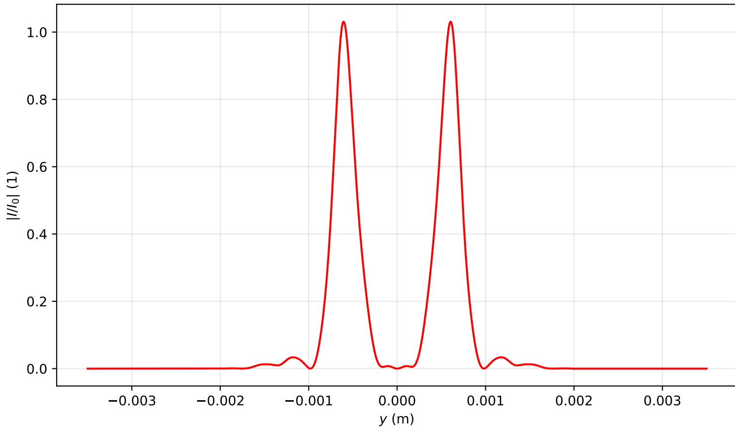
Intensity profile I(x=0, y, z=1.035)/I_0 , P_{in}=7.0P_{cr} , artificial time
